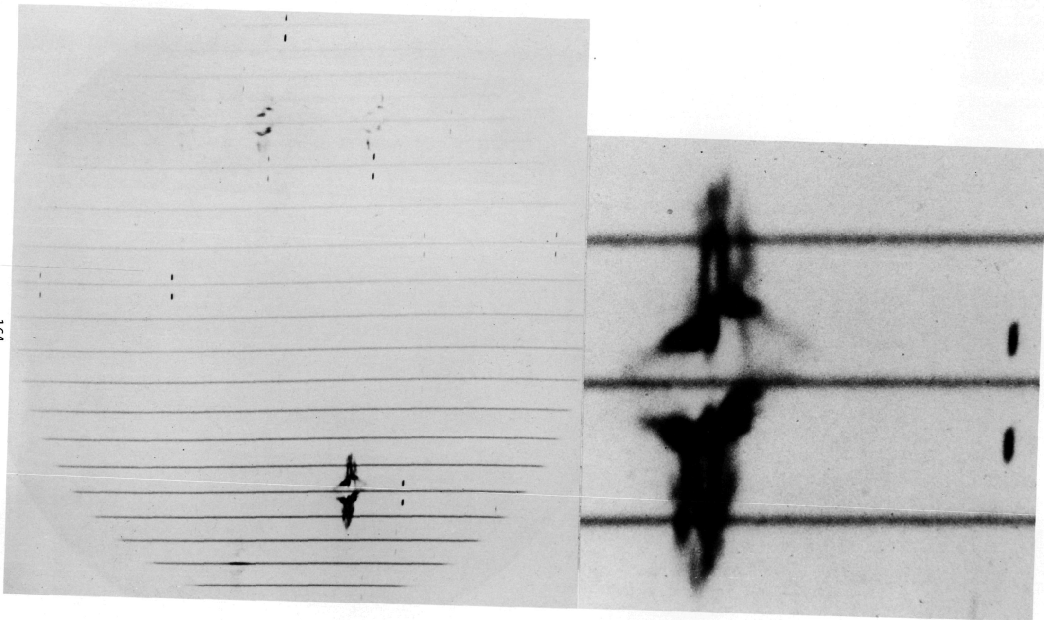
Figure 2. Echellegram of planetary nebula NGC2392. Original plate scale \sim 2.6\text{\AA}/\text{mm} at 5000\text{\AA} with seeing less than an arcsecond. The right portion is an enlargement of the 5007\text{\AA} [OIII] line with velocity dispersion approaching 200\text{ km/s} .
